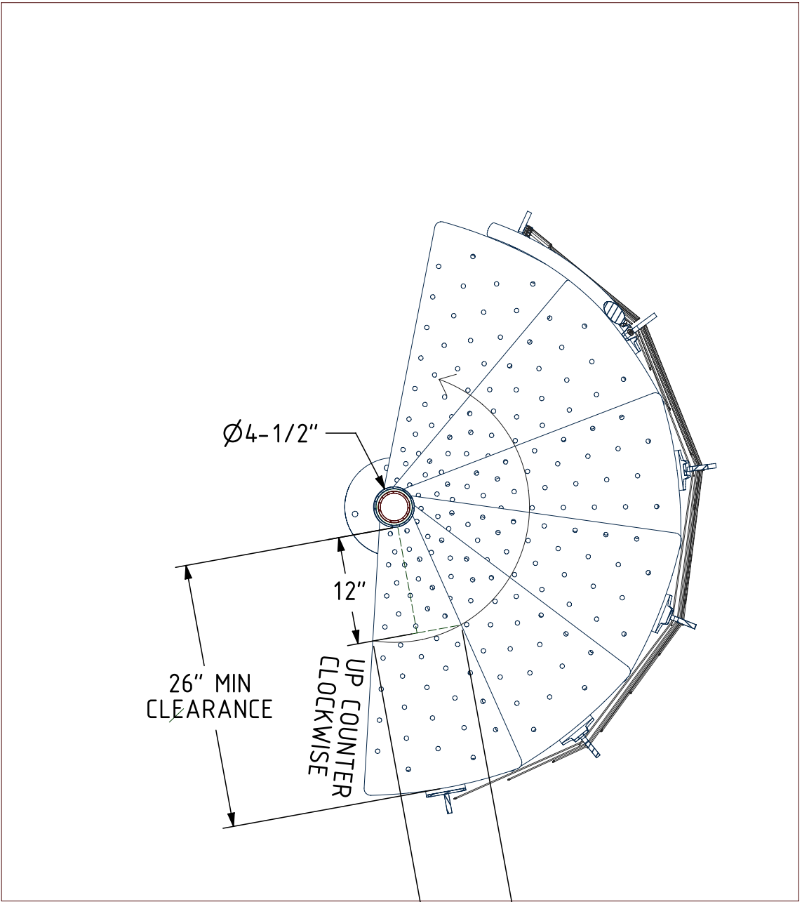
SECTION G-G TREAD ROTATION DETAIL
