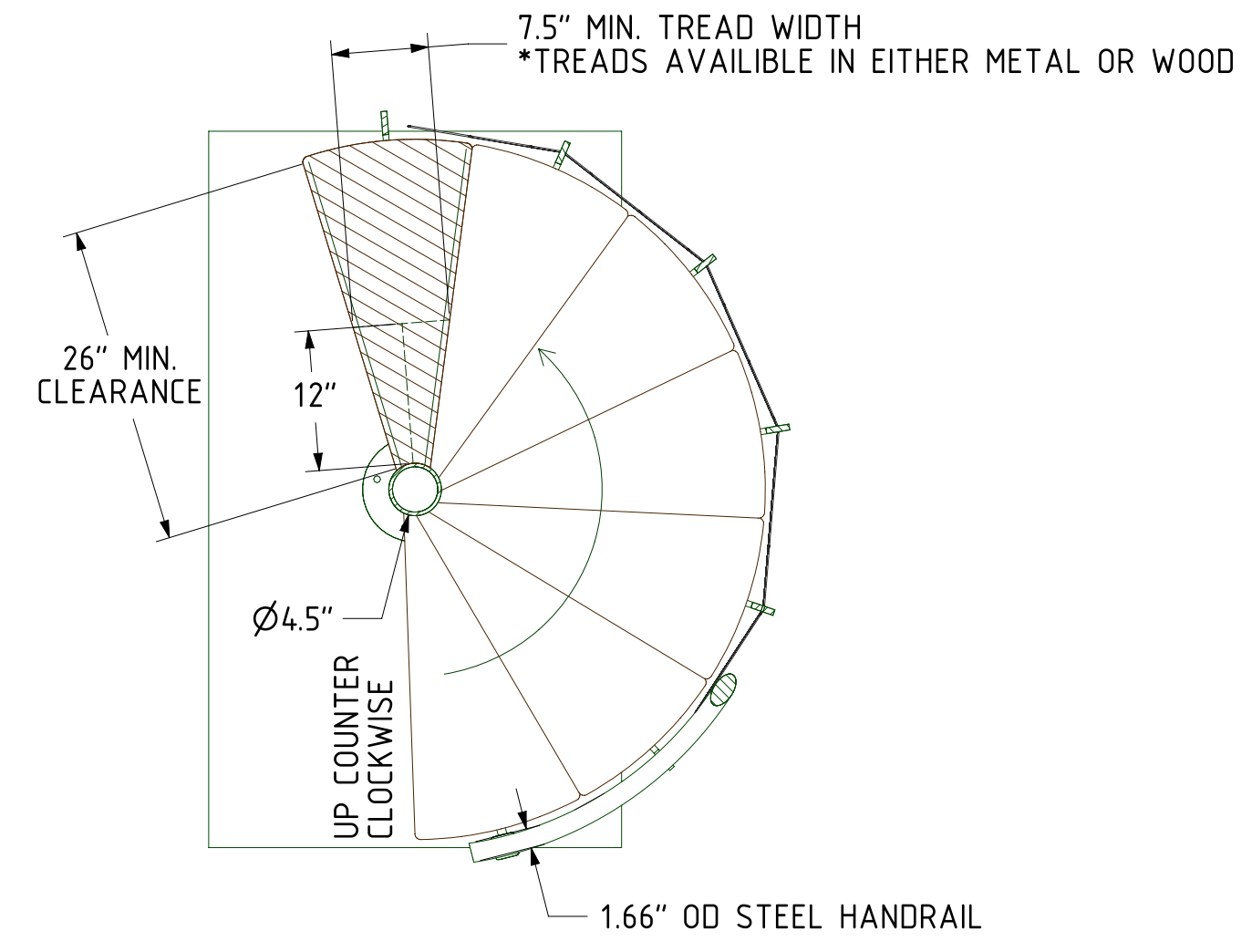
SECTION H-H TREAD ROTATION DETAIL
