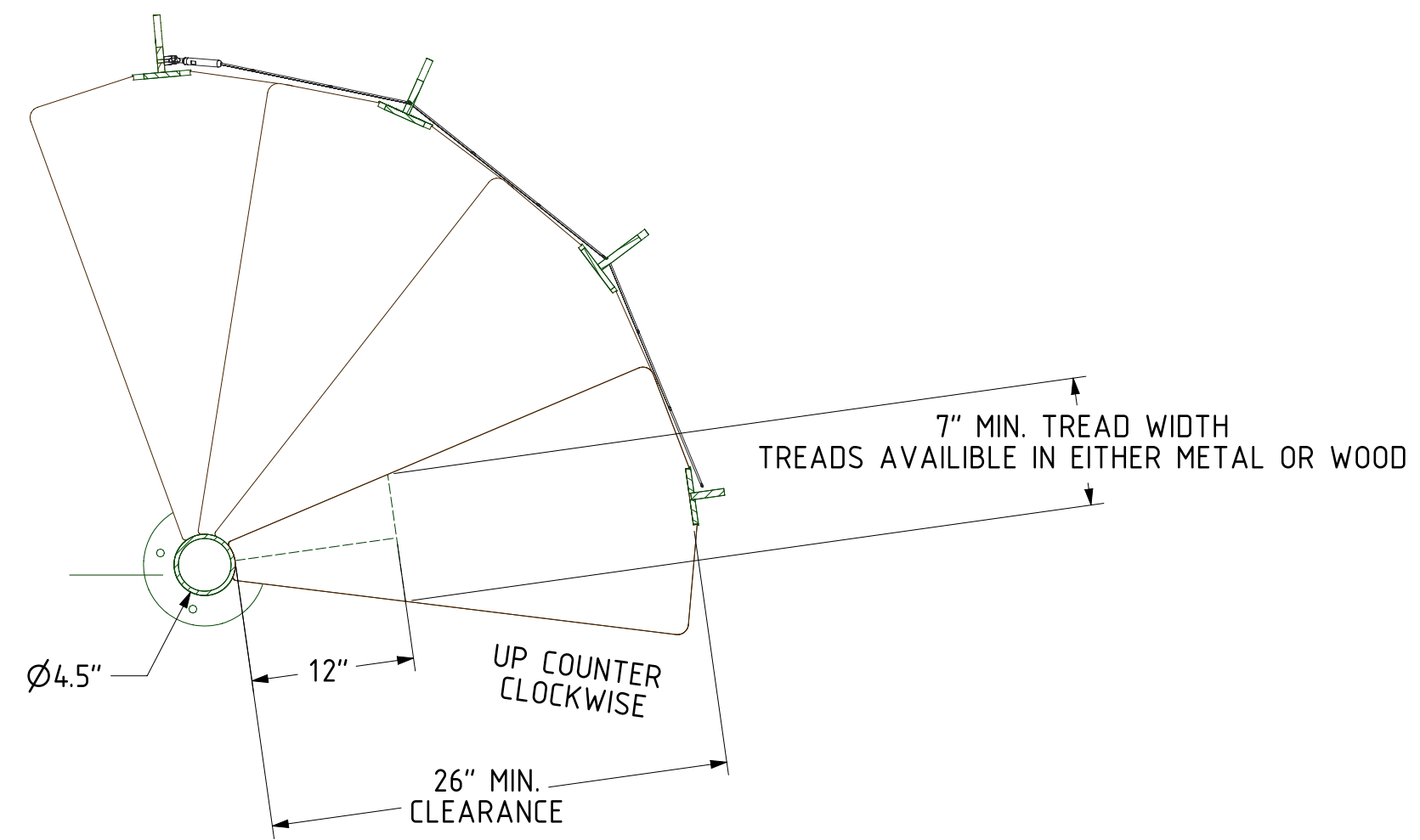
SECTION A-A TREAD ROTATIONAL DETAIL
